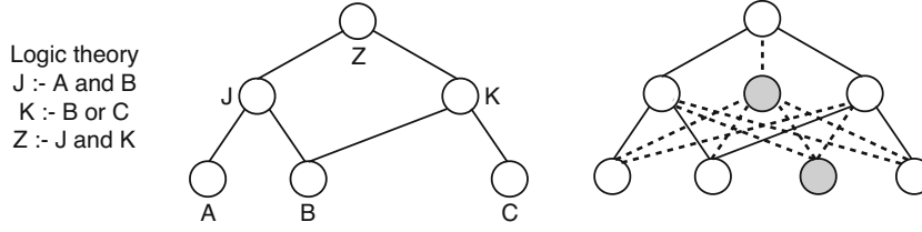
Fig. 1. Example of KBANN. A logic theory (left) is translated into a neural network architecture with conveniently initialized weights (center), further extended with additional nodes and links, which can capture hidden or unknown dependencies (right). Logical and/or functions can be modeled with appropriate weight and bias initializations.
