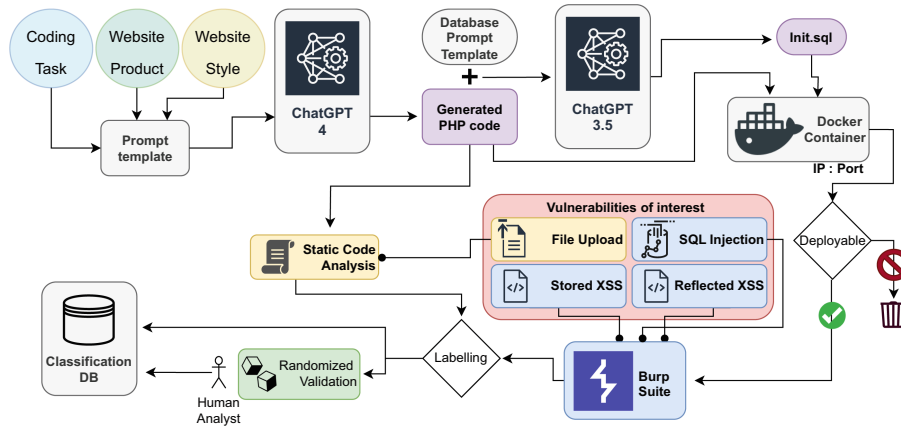
Fig. 1. Dataset Generation and Vulnerability Labelling Methodology
