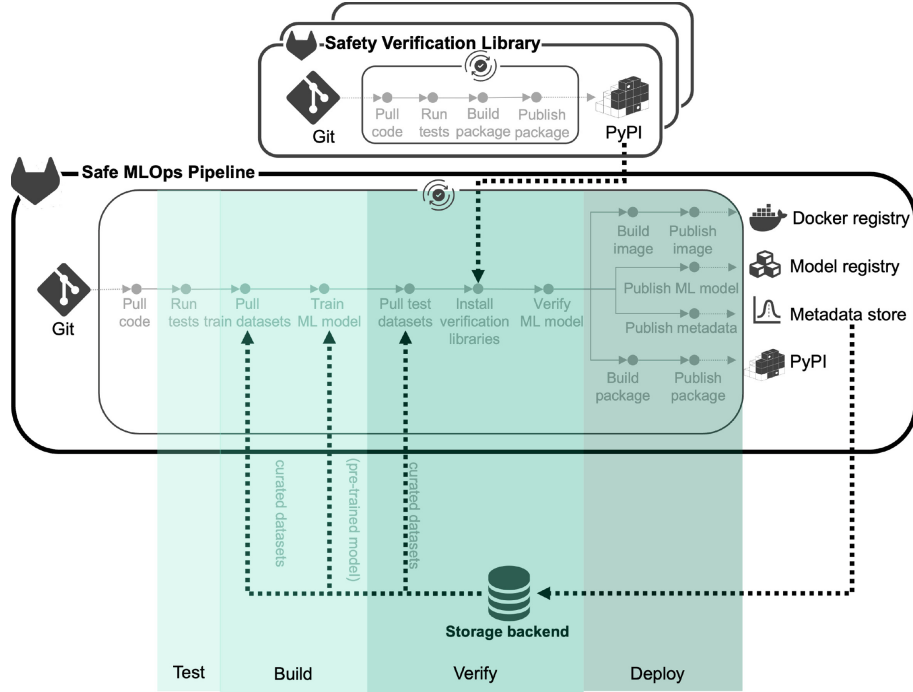
Fig. 2. Safe MLOps pipeline realized by Git-centric methods
