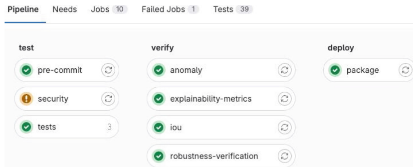
Fig. 6. Stages and jobs executed by the safe MLOps pipeline
