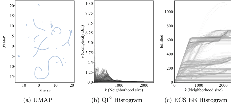
Fig. 5. Results for Data Quality Assurance on the Siemens Mobility dataset using Uniform Manifold Approximation and Projection (UMAP) [17] representation (Fig 5a), QI 2 (Fig 5b) and ECS (Fig. 5c).
