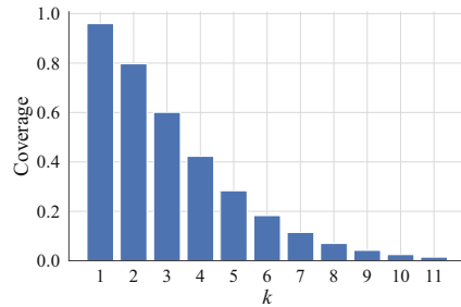
Fig. 4. Results of k -projection coverage for different values of k .
