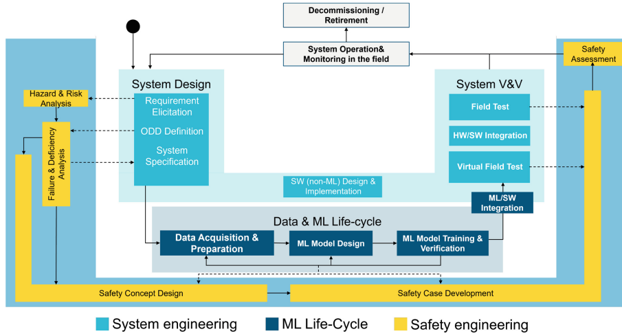
Fig. 1. Safe MLOps Process for ML-based ADS Systems
